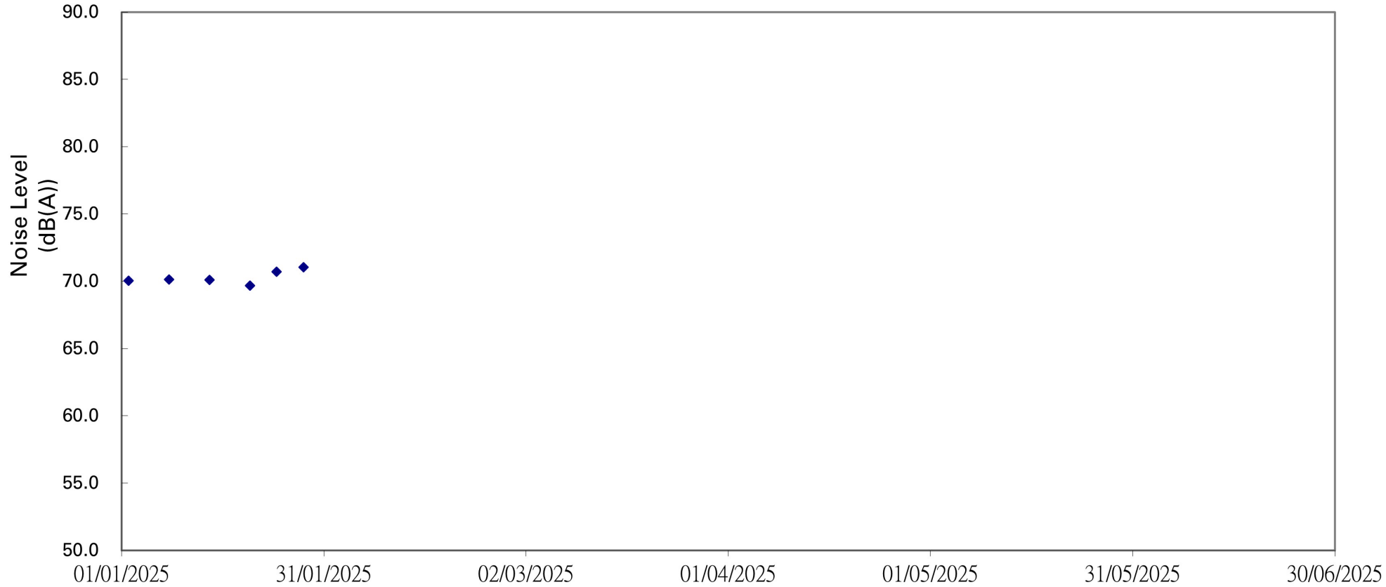
Noise Level (Leq 30 mins) dB(A) Vs Date for Location W-N18
